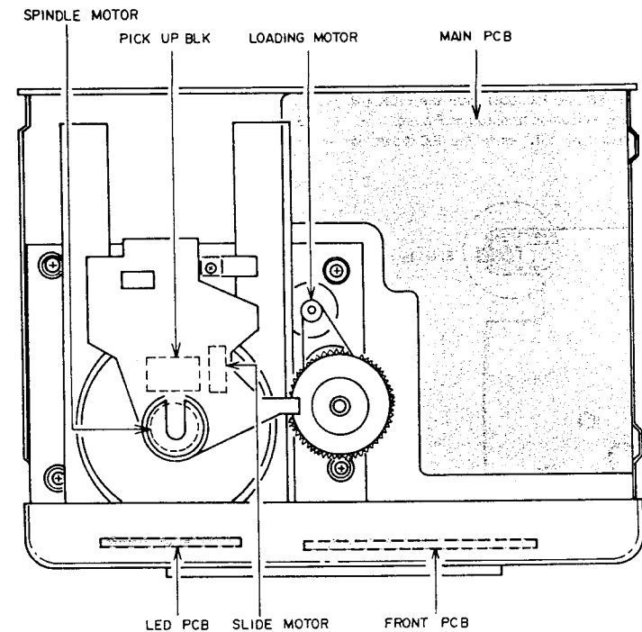
Fig. 2-1 Top view
